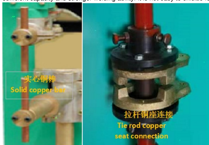
5. Solid conductive copper rod with good conductivity. The pull rod is connected with copper base, 380V current is connected, stable and durable. Transformer red copper coil and high-grade silicon steel sheet. The transformer has strong current, sufficient capacity and stronger welding ability. It is not easy to oxidize for a long time and the welding is more stable.
